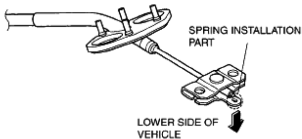
Fig. 25: Installing Parking Brake Cable Courtesy of MAZDA MOTORS CORP.
