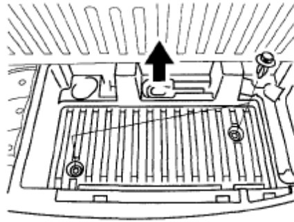
Fig. 70: Identifying Trunk Box With Clips MAZDA MOTORS CORP.
